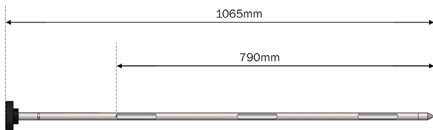
Mod. B-1000 1 m (39.37 in)
